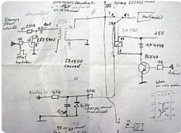
Circuit diagram
