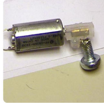
The unbalanced motor measures motion (shaking) and vibrates (motor, listerklemme, soldered screw)
