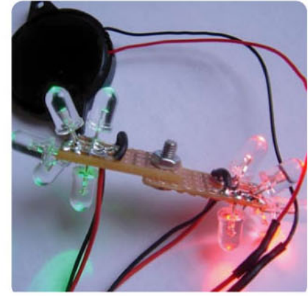
Piezo-speaker and leds
